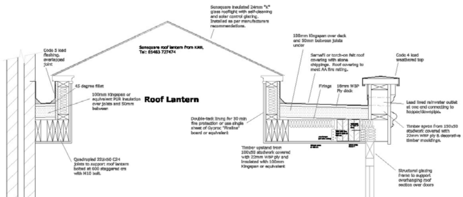
Section through Orangery showing roof lantern detail
