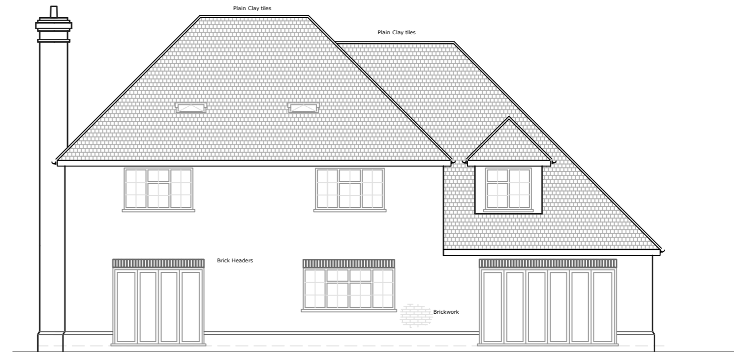
Rear Elevation
